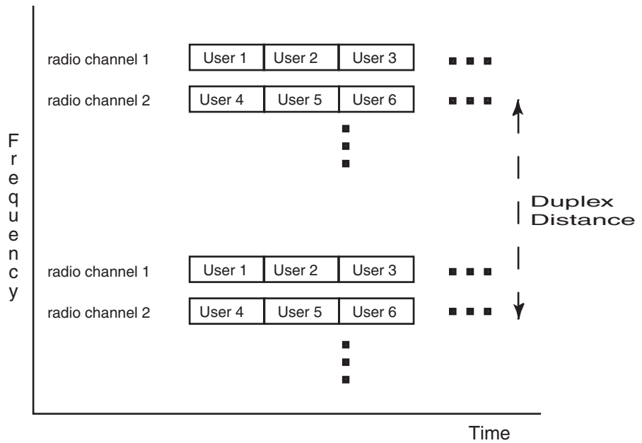
Figure 1-8 TDMA.
